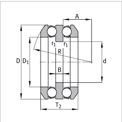
542, 543, centering seat ring
