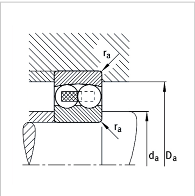
Installation dimension:
