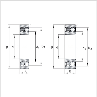
Conical hole, conical hole seal 2RS
