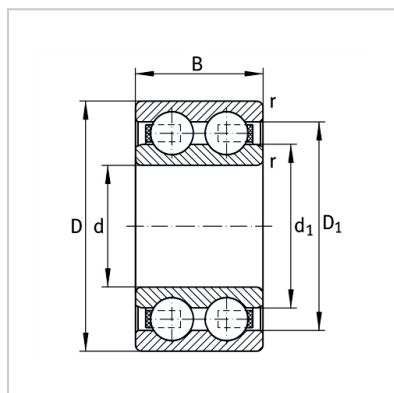
Double row
