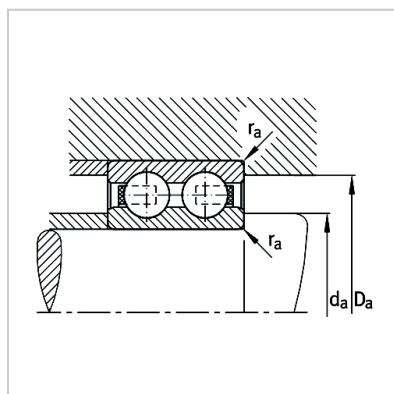
Installation dimension:
